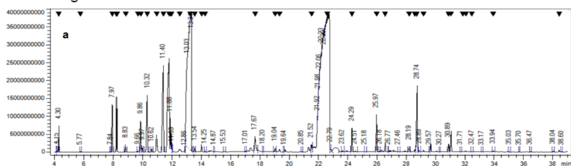
Chromatogram
